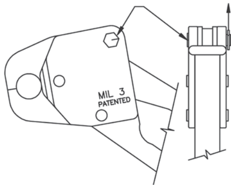
Figure 1: Back Pin Remove Retaining Clip
